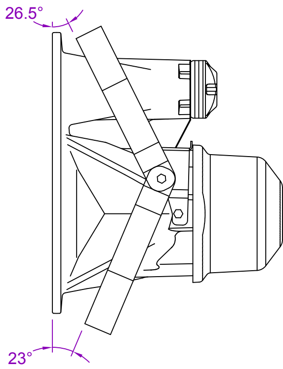
Yoke allows for \approx 230^\circ of rotation
